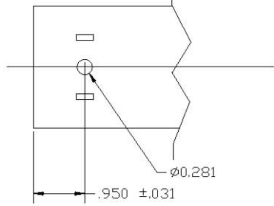
PUNCHED HOLES DETAIL
